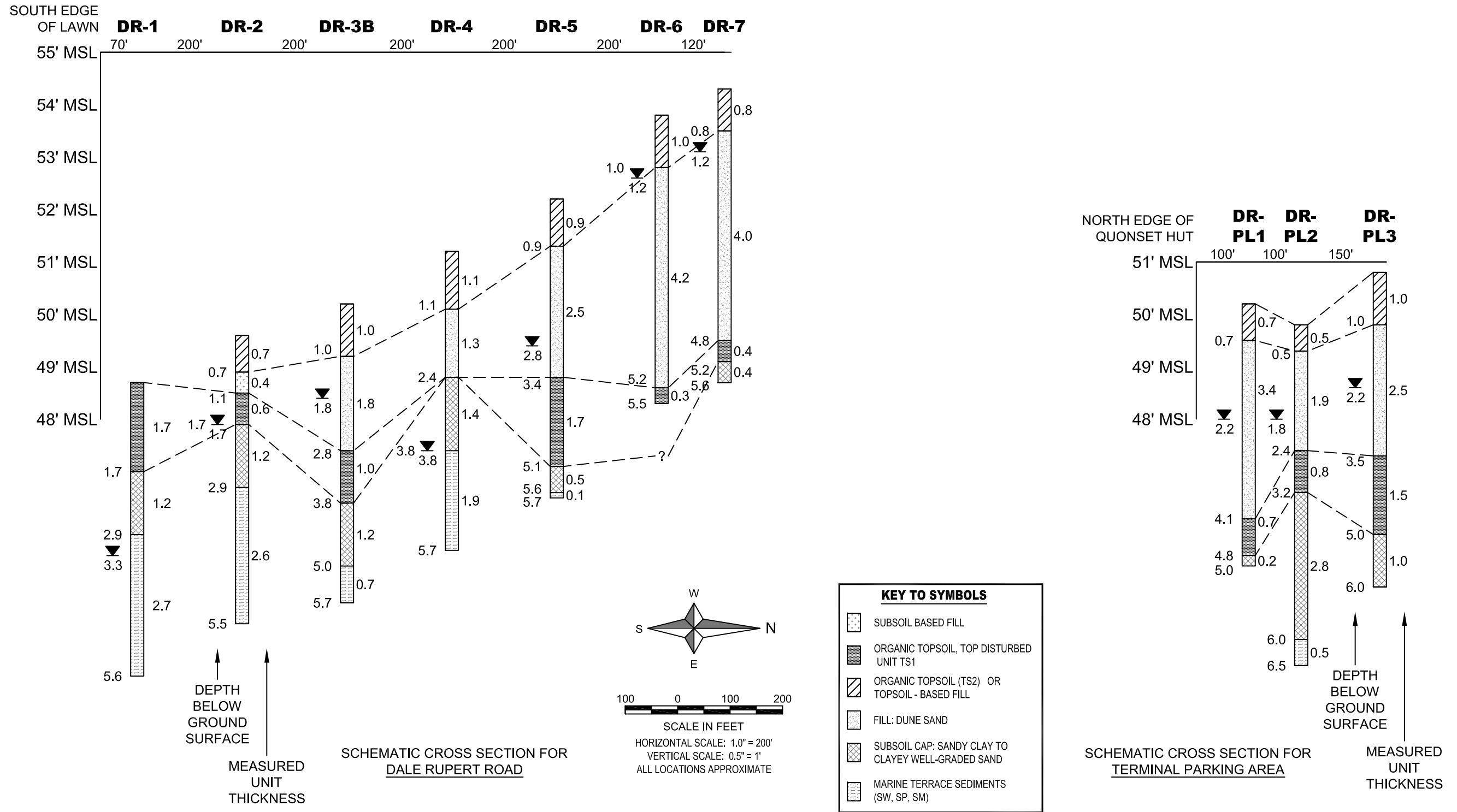
Figure 4. Schematic cross-section through BGC boreholes for Dale Rupert Road and terminal parking area. See text for discussion. Groundwater table shown as of the day we drilled the boreholes. See Figures 2 and 3 for locations.
